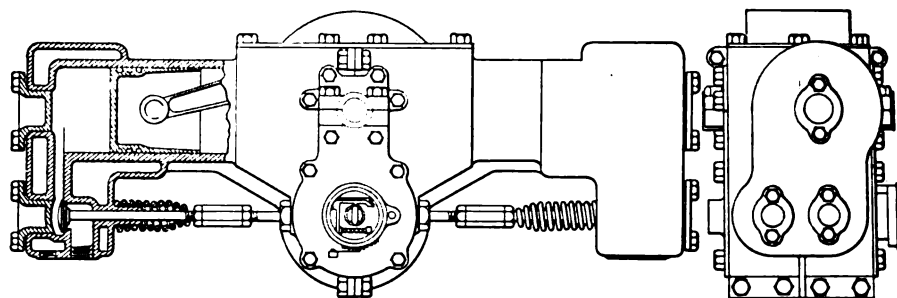
PART-SECTIONAL SIDE AND END DRAWINGS OF "MODEL" OPPOSED ENGINE.
